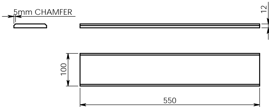
⑩ AXLE SUPPORT COVER x 2pcs (scale 1:6)
