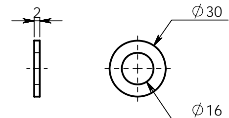
⑭ 16mm PLAIN WASHER x 8pcs
