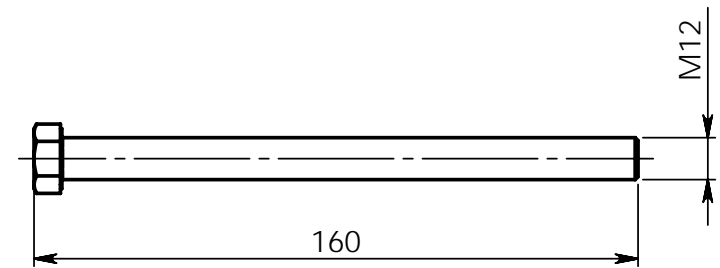
⑪ M12 HEX BOLT x 1pc
