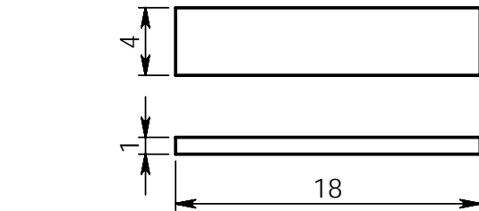
③ BACK CHASSIS MEMBER x 1pc
